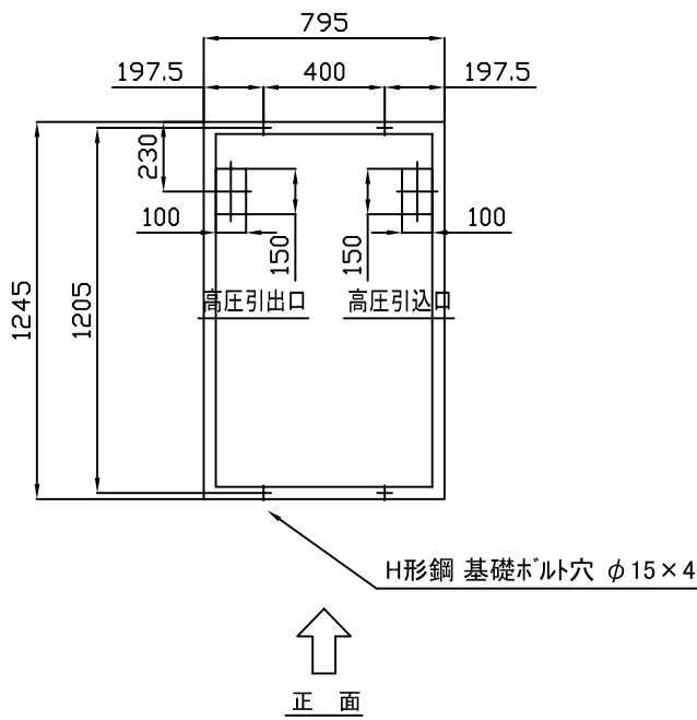
H形鋼 194×150×6×9
